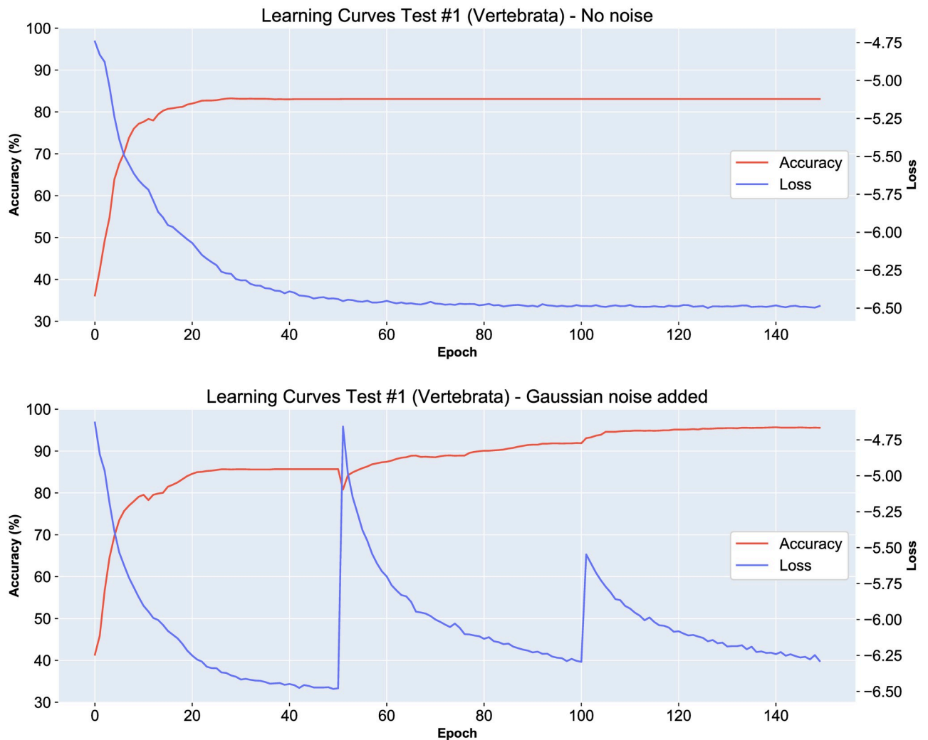
Fig 7. Learning curves for the training process of a single ANN in Step 2 of the Method, for the dataset in Test 1 (vertebrate mtDNA genomes) with (top), and without (bottom) the addition of Gaussian noise to the parameters of the networks every 50 epochs. Each graph displays the relation between the unsupervised loss function that is being minimized and the overall accuracy of the method. The true labels of the sequences are only used to evaluate the accuracy at each epoch, but they do not influence the learning process. The graph illustrates the positive effect that the periodic addition of Gaussian noise has on the prevention of convergence to suboptimal solutions, and on the classification accuracy (from \approx 82\% top, to \approx 96\% , bottom).
