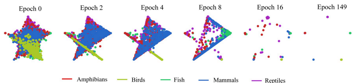
Fig 5. Learning process for the clustering of 2,500 vertebrate mtDNA full genomes into c = 5 different clusters, each corresponding to one corner of the pentagon. Each point represents a sequence, and its position indicates the probability that it is assigned to different classes. Hence, a point in the center has equal probabilities to be assigned to all 5 vertices/clusters, while a point located in a vertex has probability of 1 of belonging to that vertex/cluster. With successive epochs, the learning progresses until, at epoch 149, all sequences are correctly placed in their respective vertex/cluster. Note that points in the figure overlap if they have the same probability vector.
