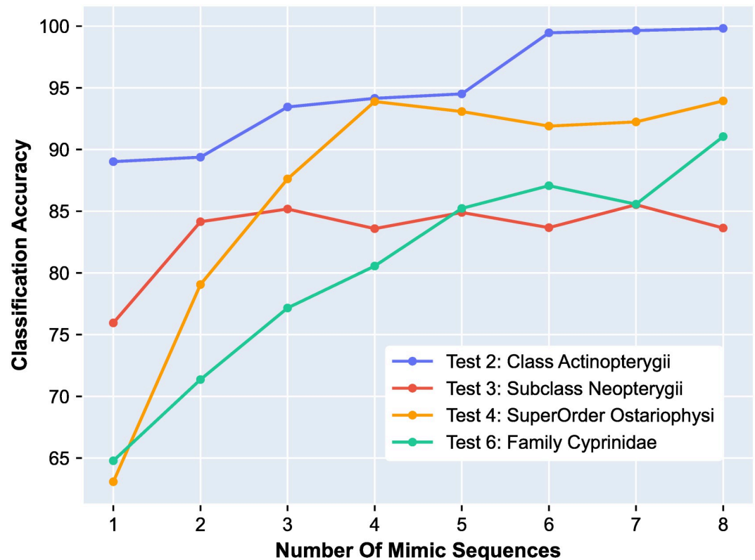
Fig 6. The effect of the number of mimic sequences on classification accuracy. Blue—Class Actinopterygii (Test 2); Red—Subclass Neopterygii (Test 3); Yellow—SuperOrder Ostariophysi (Test 4); Green—Family Cyprinidae (Test 6). In Tests 2, 4, and 6, with fewer than 150 sequences per cluster, increasing the number of mimics per sequence results in a marked increase in classification accuracy. In Test 3 (red), where the number of available sequences per cluster is sufficiently high (226 to 250), increasing the number of mimics to more than 3 does not result in an increase the classification accuracy.
