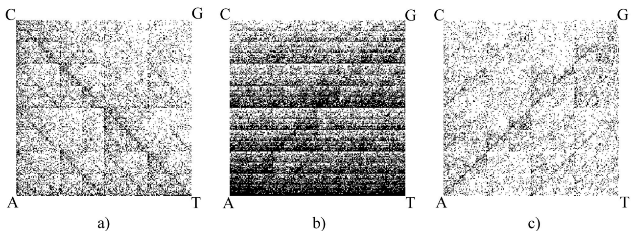
Fig 2. Chaos Game Representation of (a) the complete mitochondrial genome of Rana Chosenica (a frog), 18,357 bp—Accession ID: NC_016059.1; (b) the first 80,000 bp of the Bacillus mycoides genome—Accession ID: NZ_CP009691.1; (c) the complete genome of Dengue Virus 2 , 10,627 bp—Accession ID: GU131948.1.
